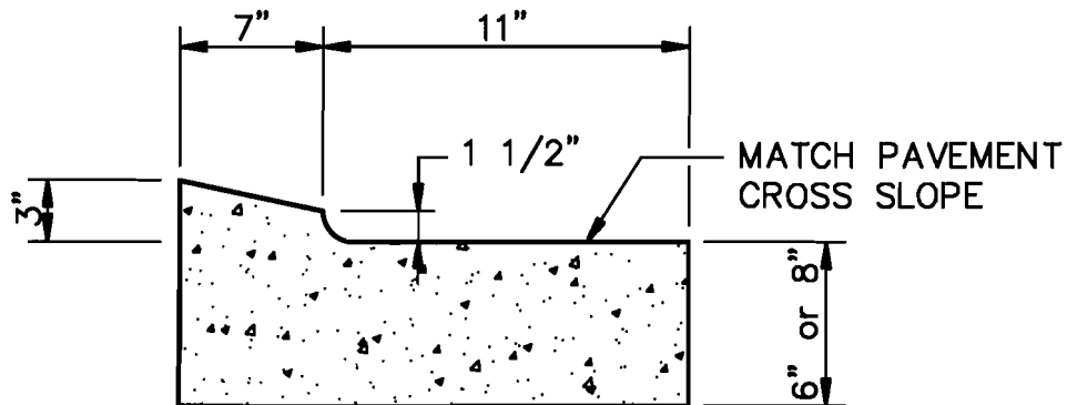
TYPE "A-18" - DEPRESSED
