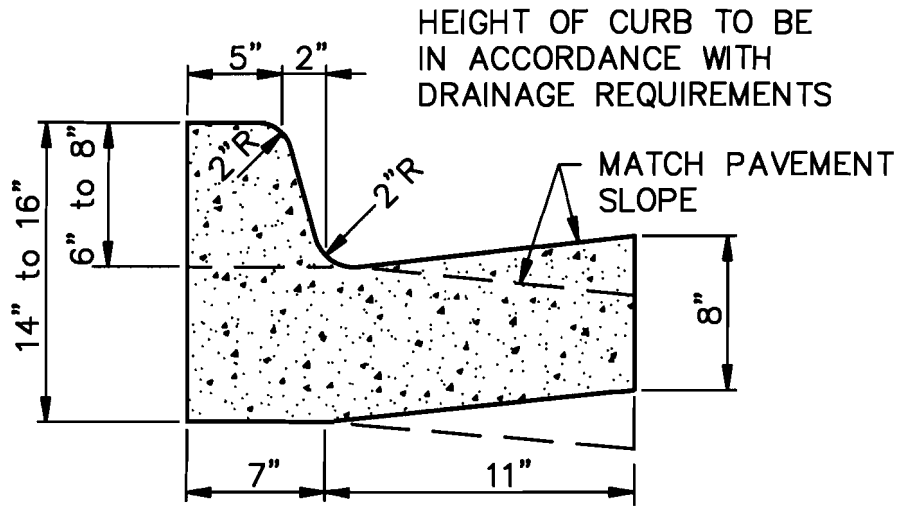
TYPE "A-18" (BARRIER) ARTERIAL STREETS
