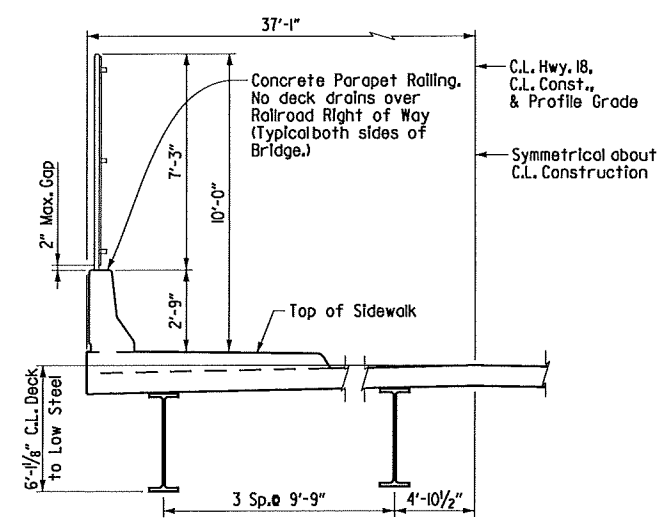
TYPICAL HALF SECTION No Scale
