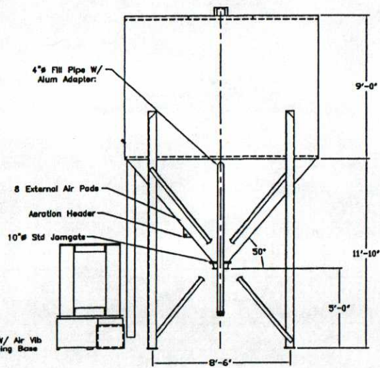
270 BARREL SILO 1080 CU/FT 50.8 TONS GROUND MOUNT DUST COLLECTOR
