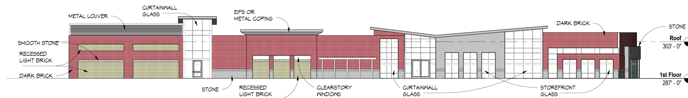
SOUTH ELEVATION
