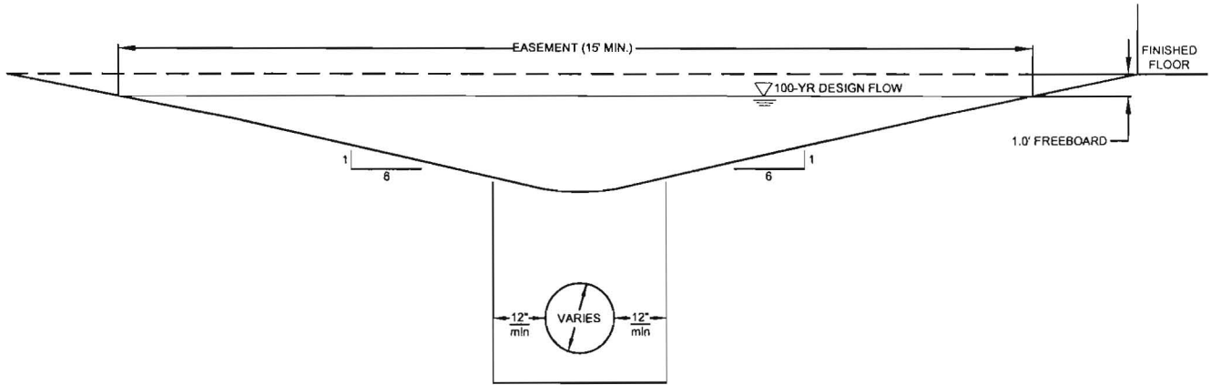
TYPICAL DRAINAGE PIPE/SWALE SECTION
