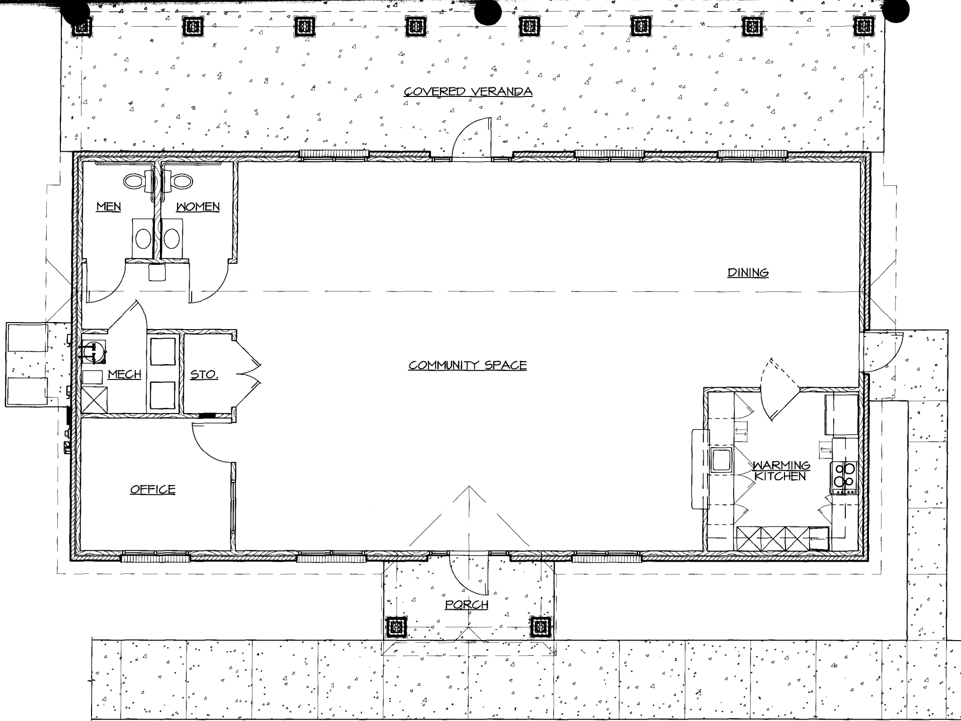
FLOOR PLAN - COMMUNITY BLDG
