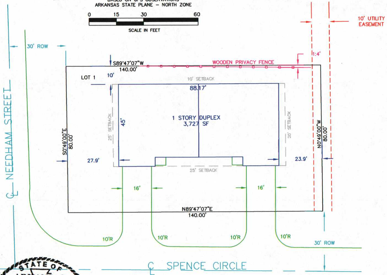
PLOT PLAN
