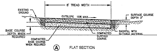
① TYPICAL TRAIL CROSS SECTIONS N.T.S.
