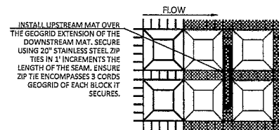
① ABUTMENT METHOD FOR SEAMS PERPENDICULAR WITH FLOW N.T.S.
