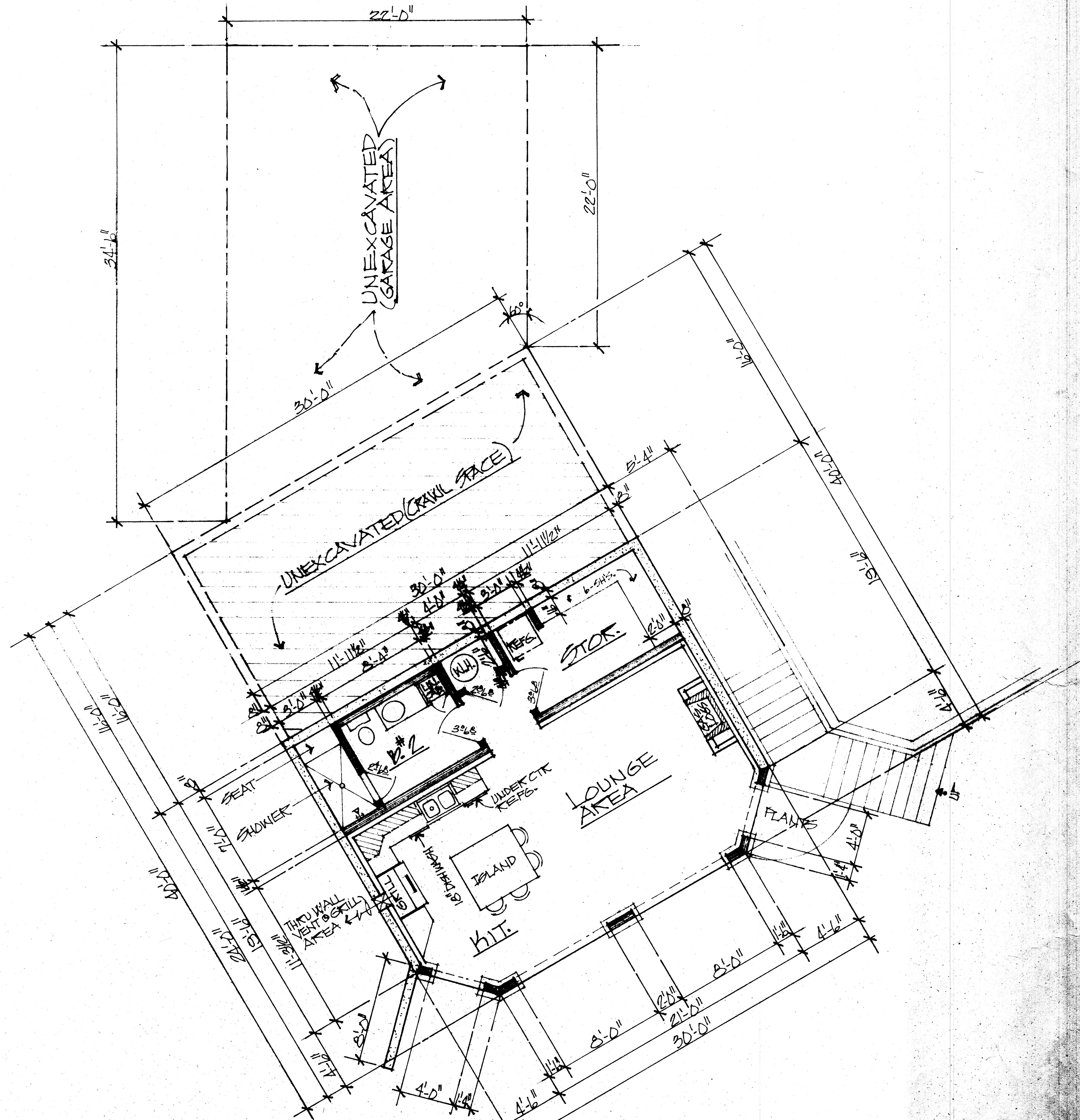
FIRST FLOOR PLAN — SC: - 1/4" = 1'-0"
