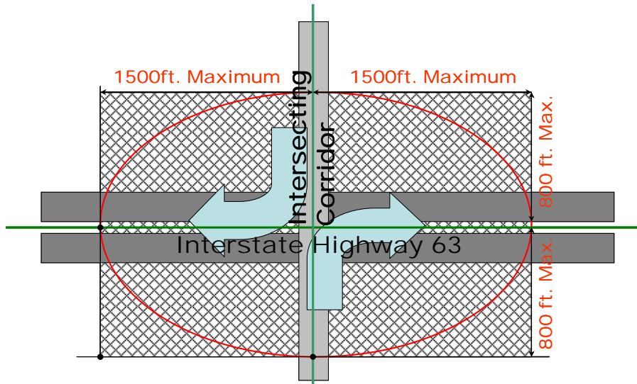
Figure 11.8.3: High-rise Sign Location Limit (Allowed within shaded area only)
