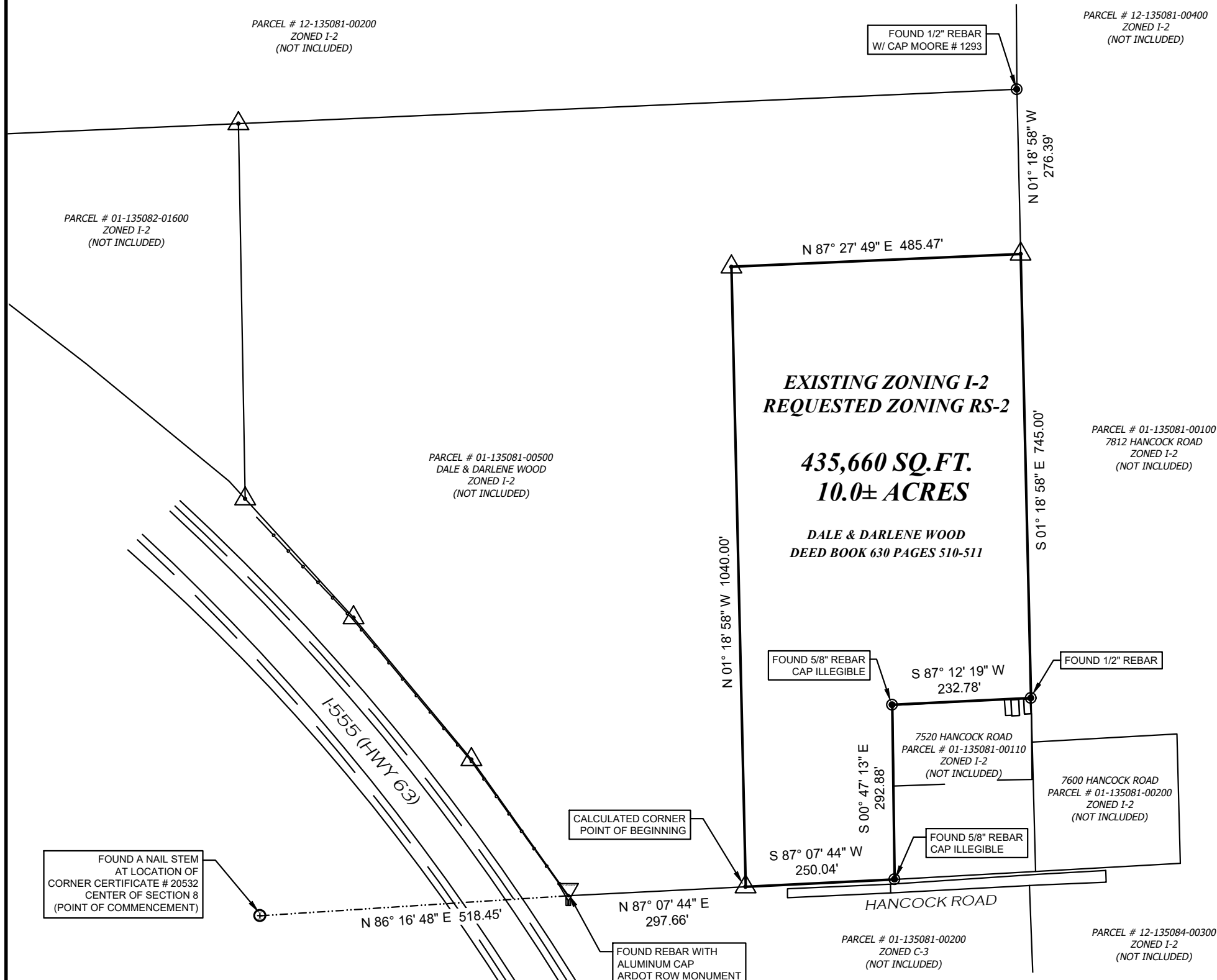
SURVEYOR'S NOTES: 1. SURVEYOR HAS MADE NO INVESTIGATION OR INDEPENDENT SEARCH FOR EASEMENTS OF RECORD OR ANY OTHER FACTS THAT AN ACCURATE TITLE SEARCH MAY DISCLOSE. 2. THE FOLLOWING DOCUMENTS WERE USED AS REFERENCES FOR THIS SURVEY: a. DEED - HANCOCK TO WOOD, CRAIGHEAD COUNTY COURTHOUSE, BOOK 630 PAGES 510-511, DATED 07/30/2002. b. RIGHT OF WAY MAP, ARKANSAS HIGHWAY DEPARTMENT, JOB # 10936 c. SURVEY - JOHN STUCKY, BY. D. MOORE #1293, ARK. DIV. OF SURVEYS, DOCUMENT # 202202246763, DATED 05/05/2021. d. DEED - WALKER, CRAIGHEAD COUNTY COURTHOUSE, BOOK 703 PAGES 68-69, DATED 08/01/2005.
