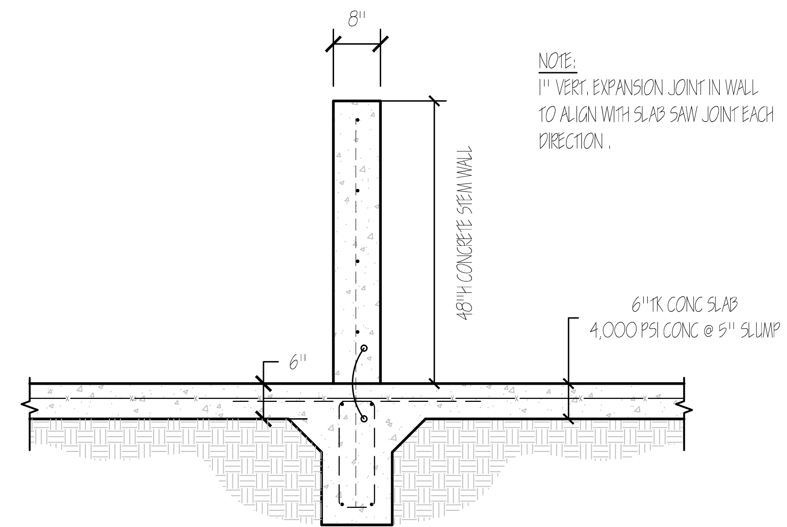
② SECTION AT INTERIOR WALL 3/4"=1'
