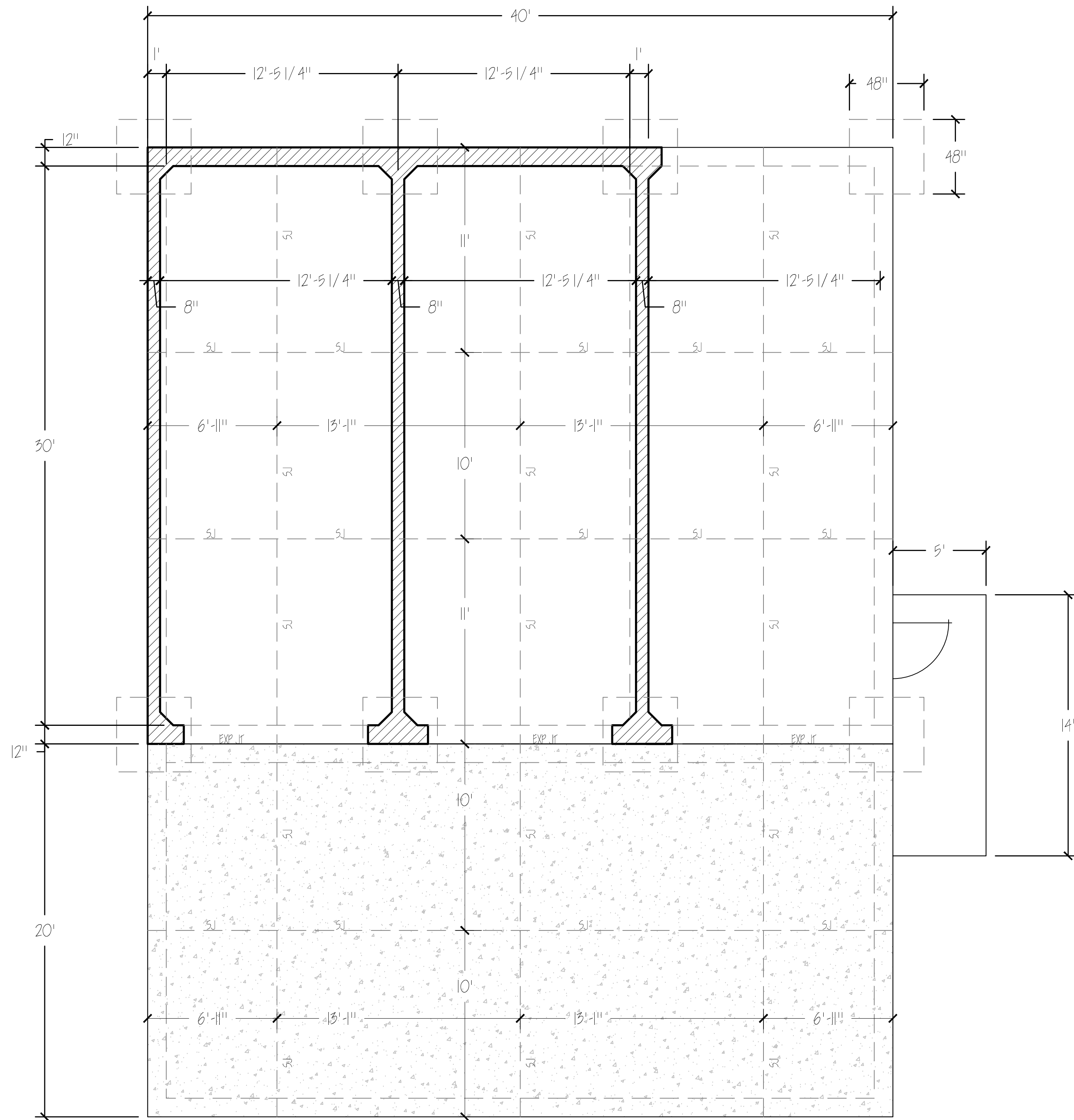
FOUNDATION PLAN 1/4"=1'
