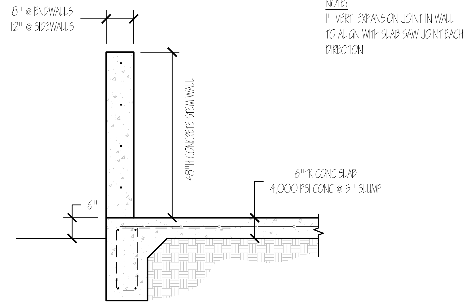
① SECTION AT EXTERIOR WALL 3/4"=1'
