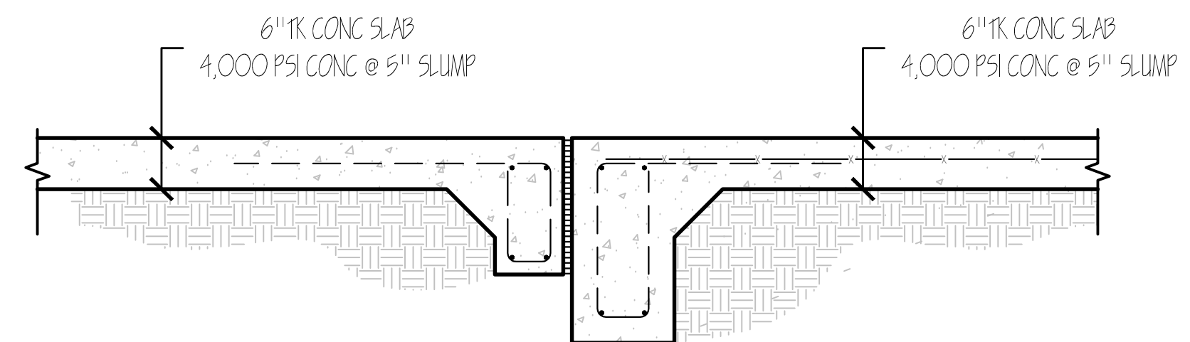
③ SECTION AT DOOR 3/4"=1'
