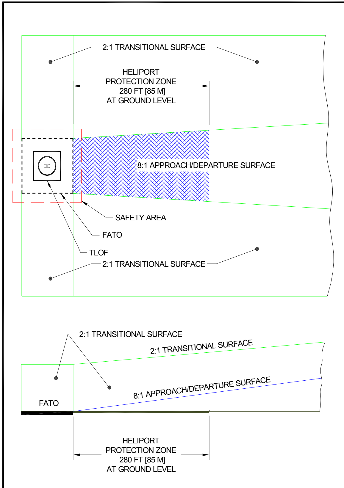
Figure 4–11. Heliport Protection Zone: Hospital
