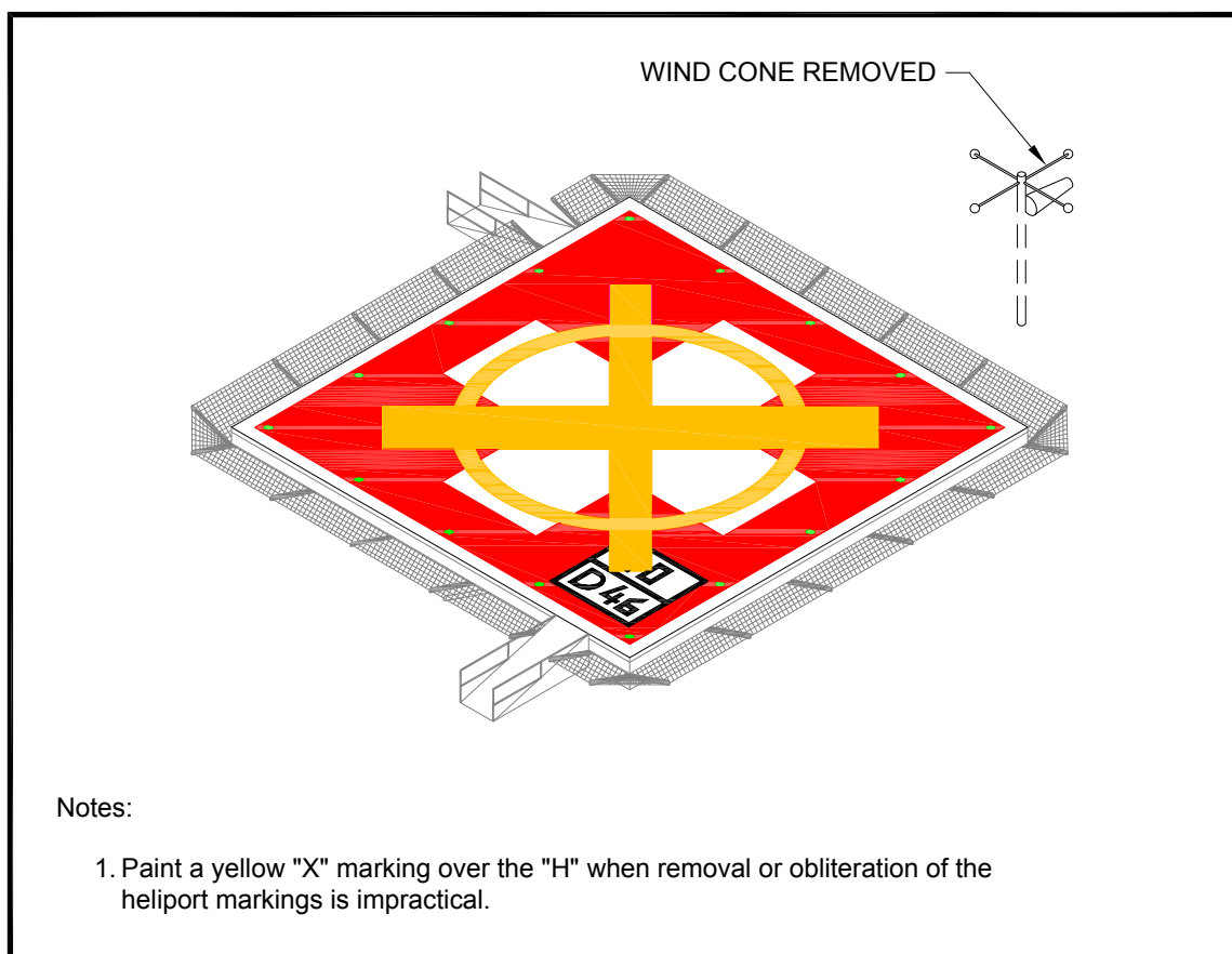
Figure 4–27. Marking a Closed Heliport: Hospital
